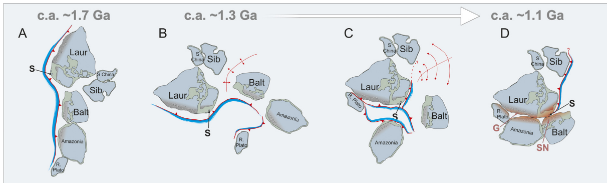
Fig. 1. Schematic plate reconstruction of the amalgamation of Rodinia from 1.7 Ga to 1.1 Ga based on the reconstructions of Li et al. (2008) , Cawood and Pisarevsky (2017) and Martin et al. (2020) . Laur = Laurentia, S = Scotland, S China = South China Craton, Sib = Siberian craton, Balt = Baltica, R. Plata = Rio de la Plata craton, G = Grenville orogeny, SN = Sveeno-norwegian Orogeny. Dark blue with red trim = subduction (red teeth indicate hanging-wall side), double ended red arrows = ocean spreading, red/orange shading = ~1.1 Ga orogenesis. (For interpretation of the references to colour in this figure legend, the reader is referred to the web version of this article.)
