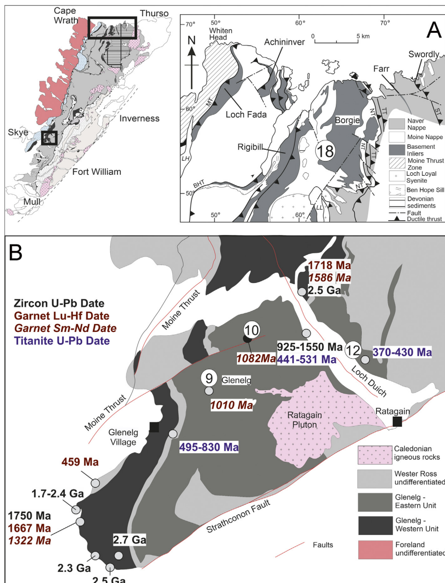
Fig. 2. Simplified map of the northern Highlands, Scotland and study areas. (A) Shows the geology of northern Sutherland and the location of the Borgie and other inliers mentioned within the text. BHT – Ben Hope Thrust, LL – Loch Loyal, MT – Moine Thrust, NT – Naver Thrust, ST – Swordly Thrust, TT – Torridale Thrust. (B) Shows the geology of the Glenelg region and the locations of samples with published data ( Storey et al., 2004, 2010; Storey, 2008 ) and locations of the samples within this study.
